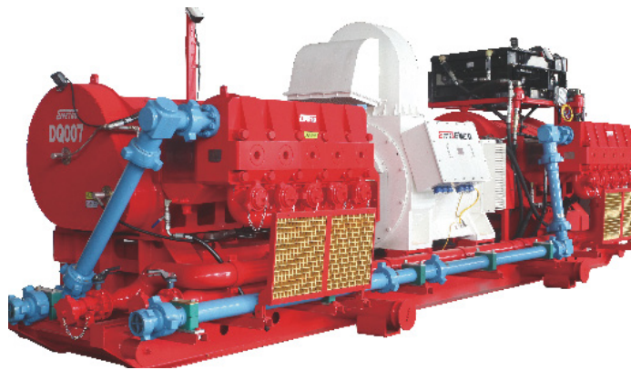
SYLQ5000Q-140D Electric Fracturing Pump Skid
